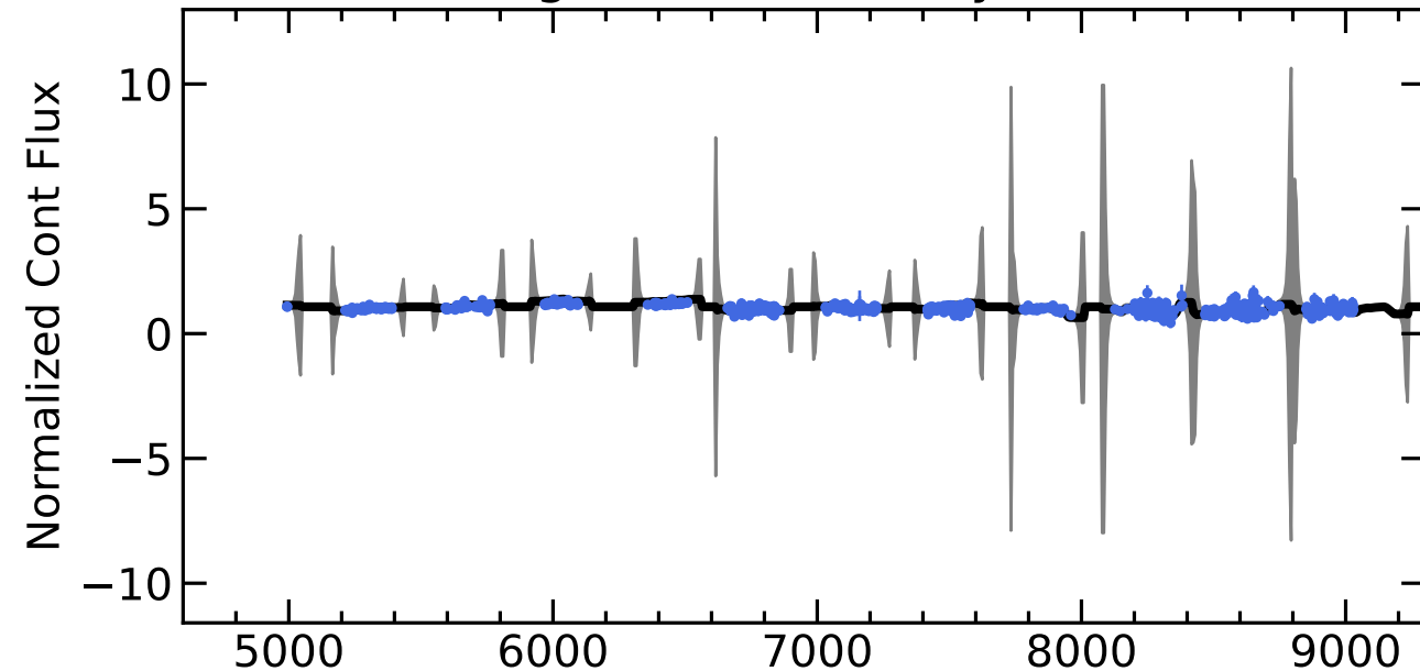
RM532 Light Curves (w/ PyROA model)
