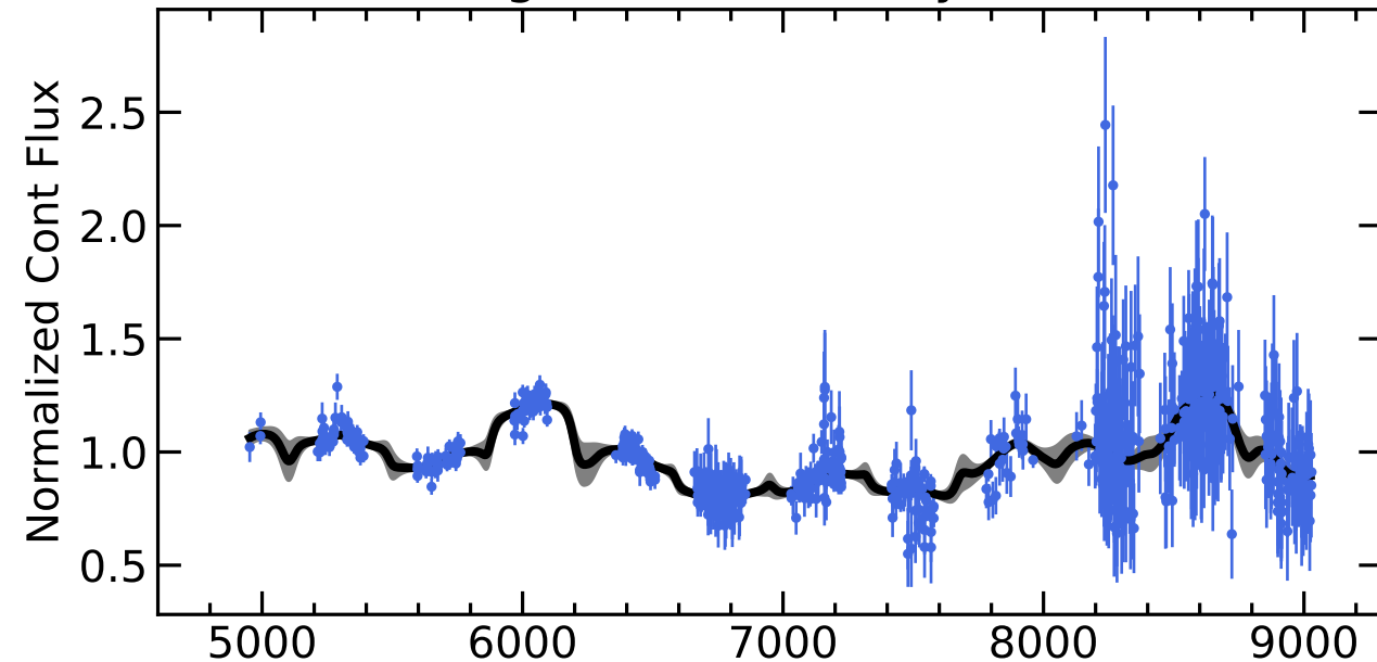
RM533 Light Curves (w/ PyROA model)
