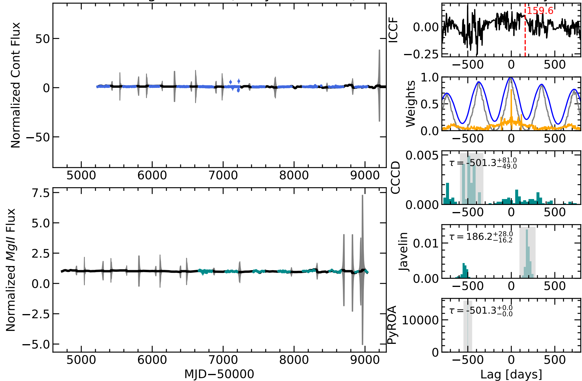
RM534 Light Curves (w/ PyROA model)
