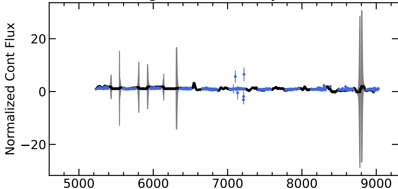
RM534 Light Curves (w/ PyROA model)
