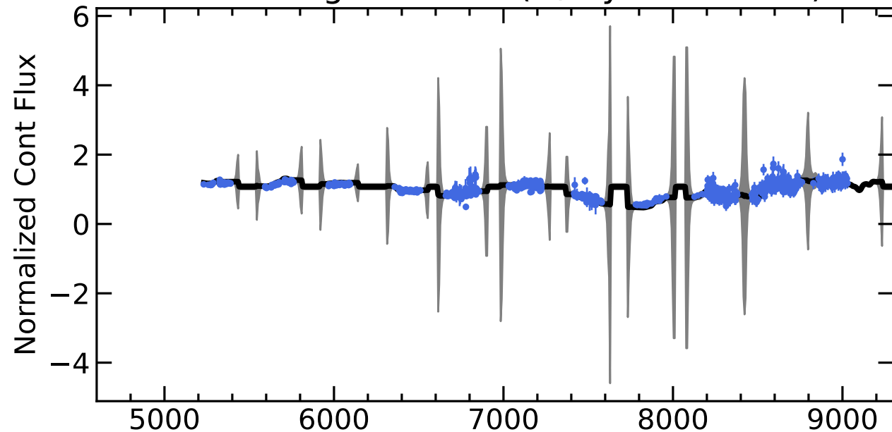
RM535 Light Curves (w/ PyROA model)
