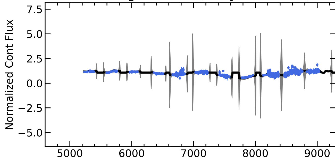
RM535 Light Curves (w/ PyROA model)
