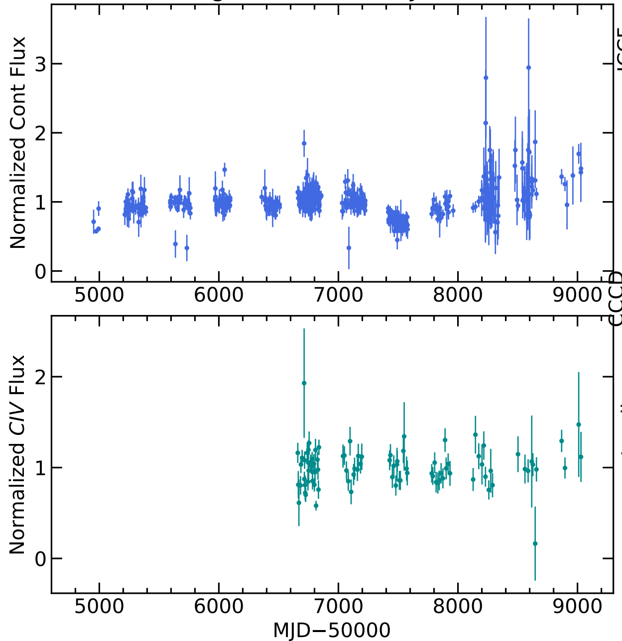
RM536 Light Curves (w/ PyROA model)
