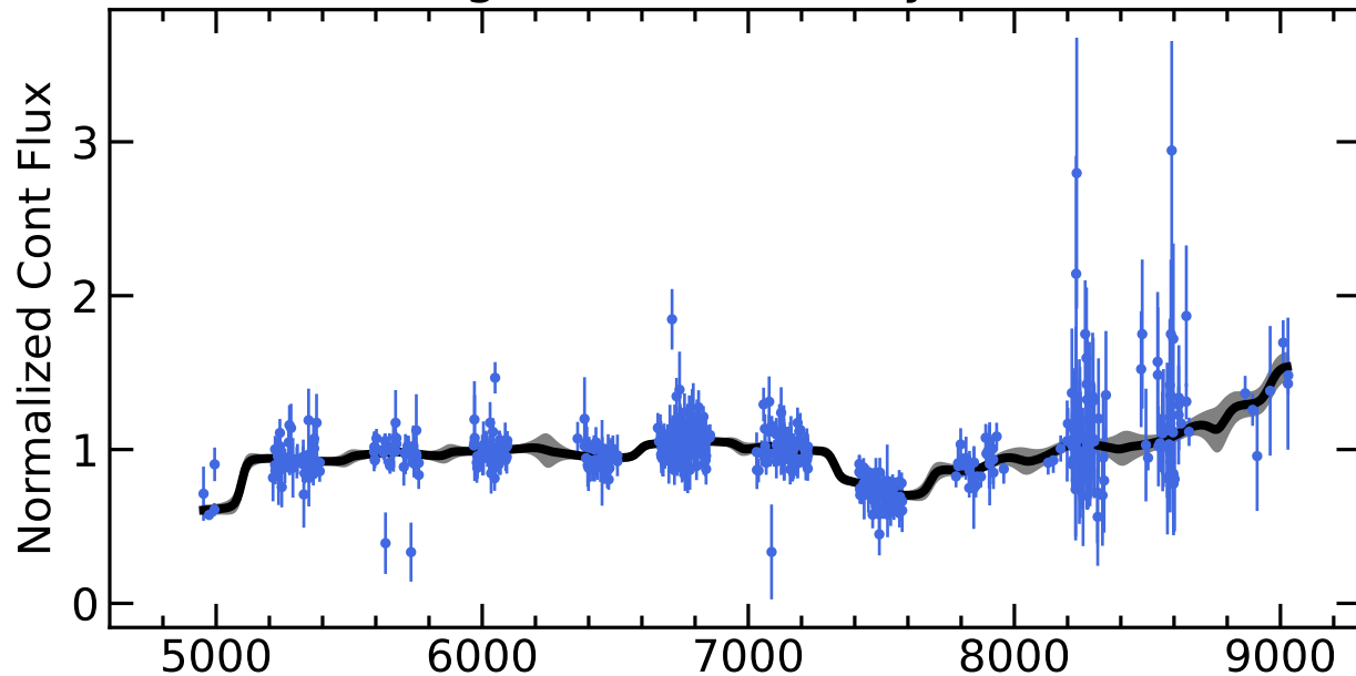
RM536 Light Curves (w/ PyROA model)
