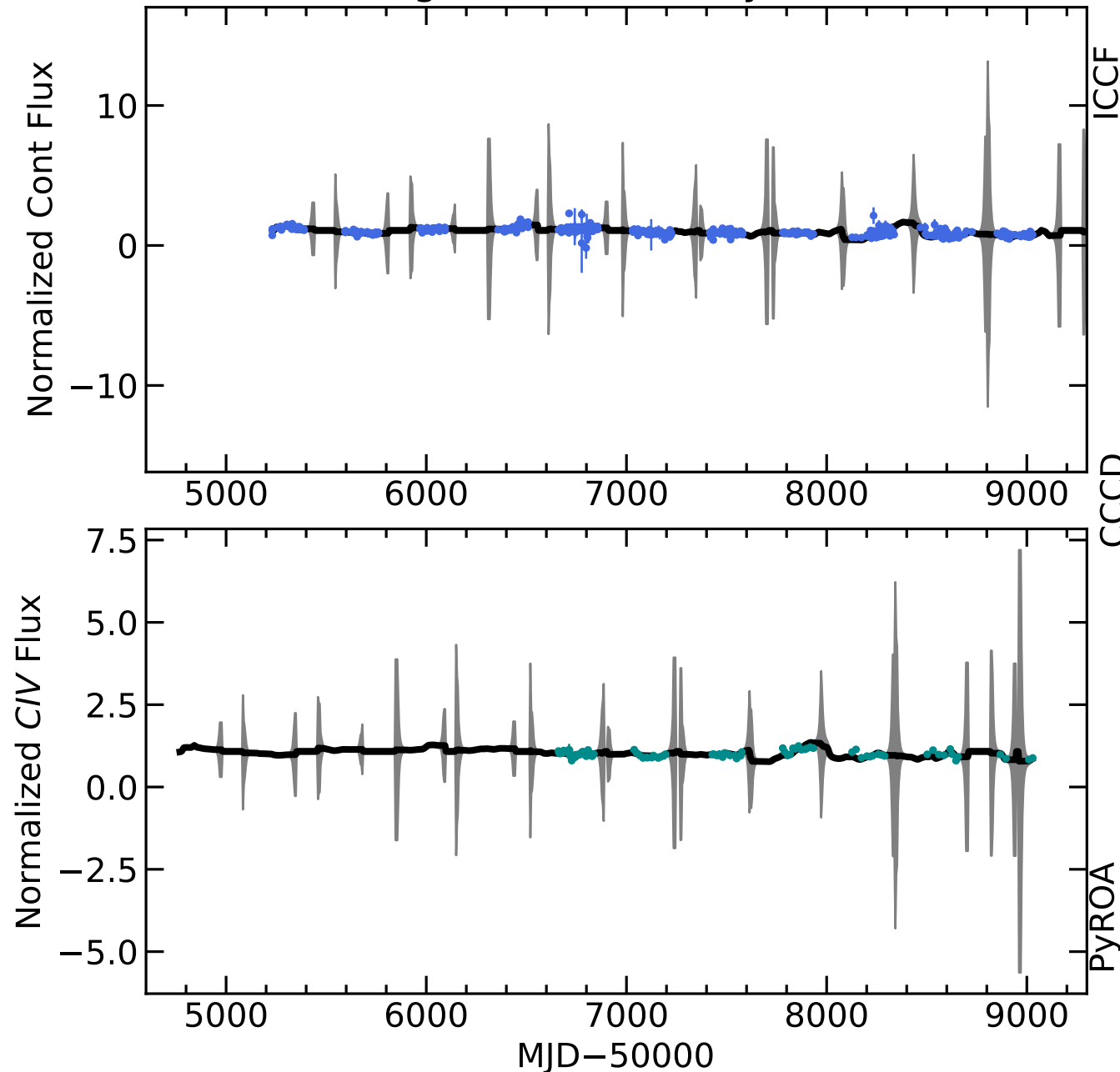
RM538 Light Curves (w/ PyROA model)
