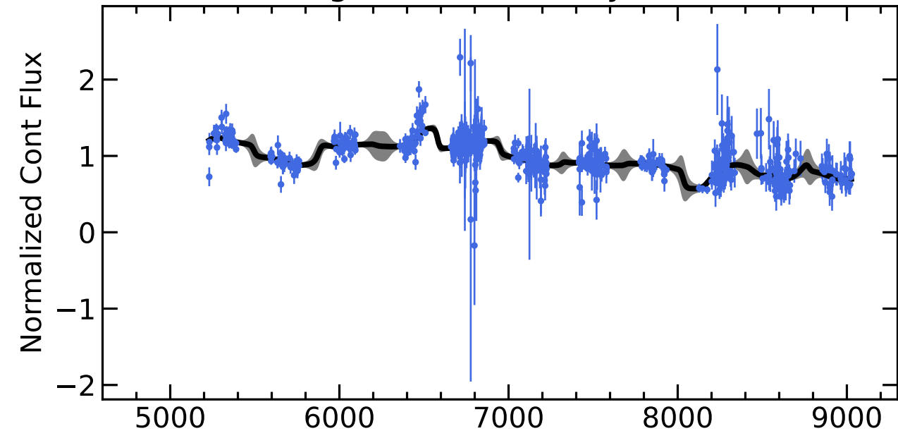
RM538 Light Curves (w/ PyROA model)
