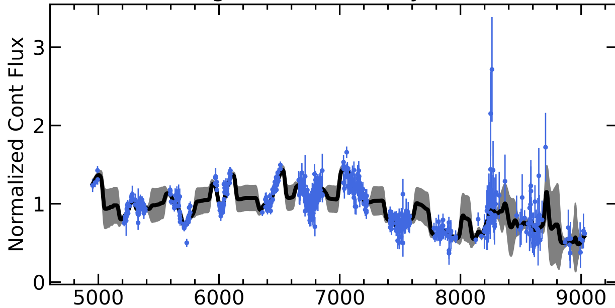
RM539 Light Curves (w/ PyROA model)
