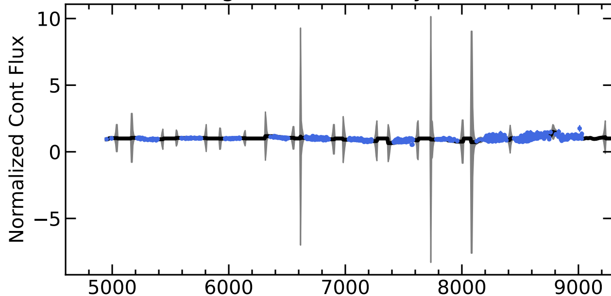
RM540 Light Curves (w/ PyROA model)
