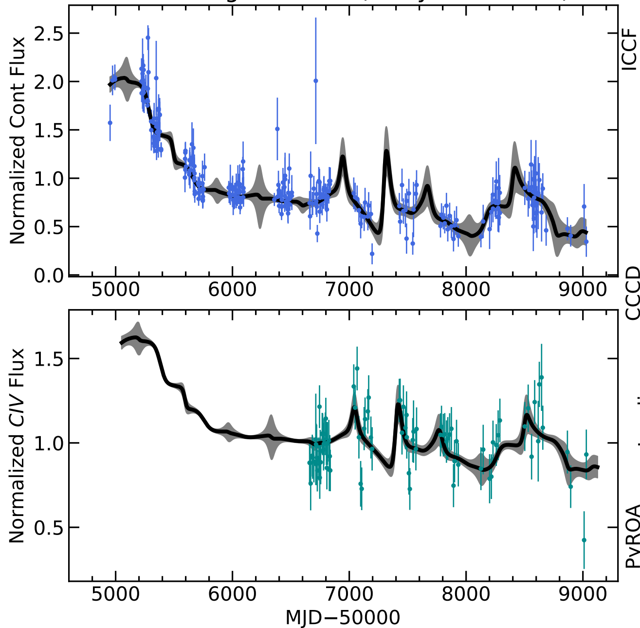
RM542 Light Curves (w/ PyROA model)
