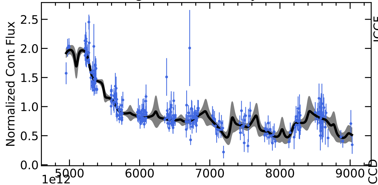
RM542 Light Curves (w/ PyROA model)
