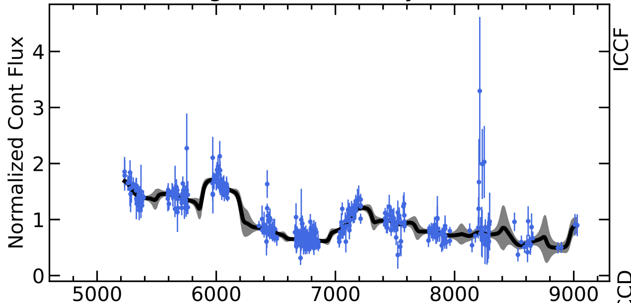
RM544 Light Curves (w/ PyROA model)
