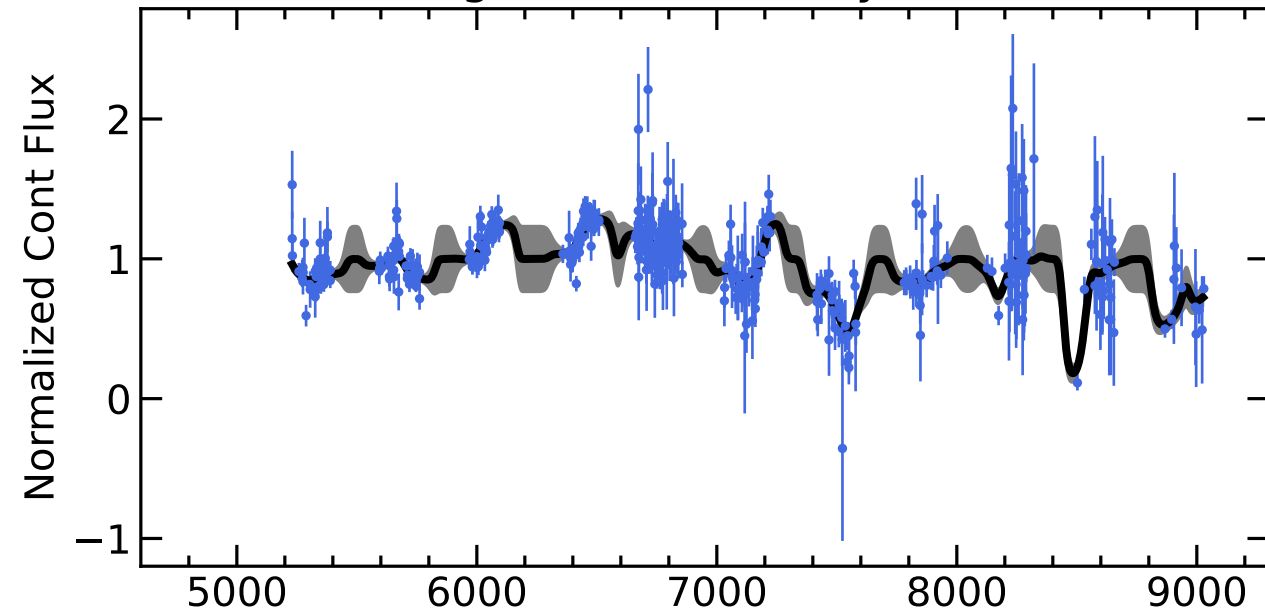
RM547 Light Curves (w/ PyROA model)
