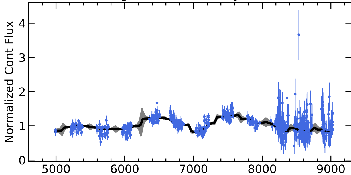
RM548 Light Curves (w/ PyROA model)
