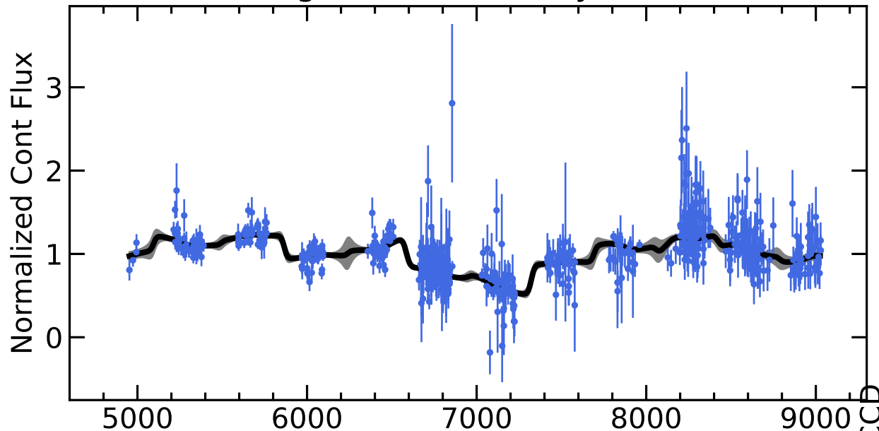
RM550 Light Curves (w/ PyROA model)
