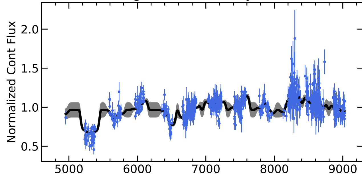
RM551 Light Curves (w/ PyROA model)
