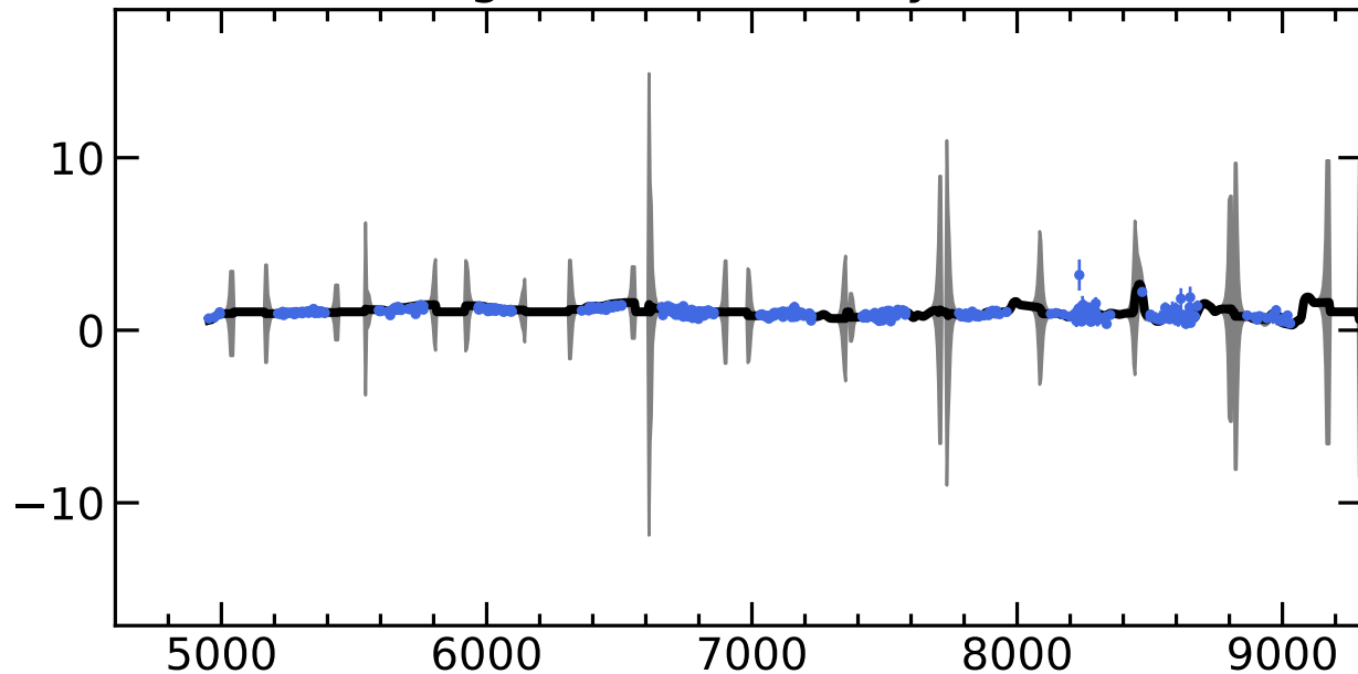
RM552 Light Curves (w/ PyROA model)
