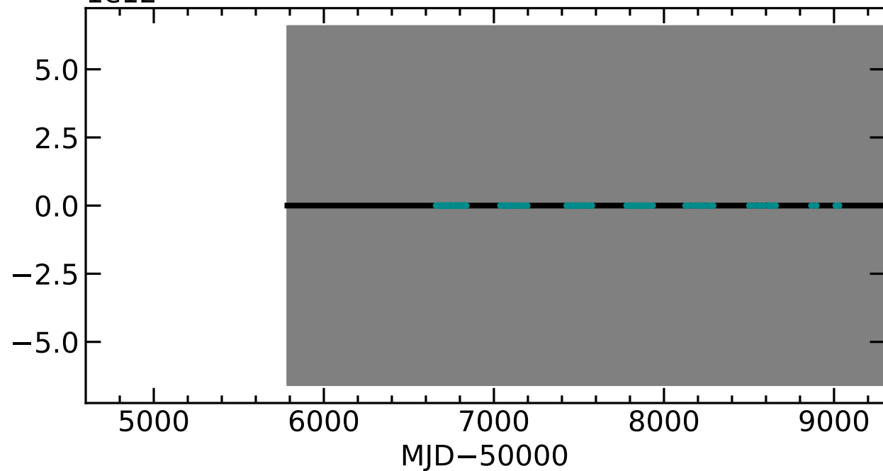
Normalized MgII Flux
