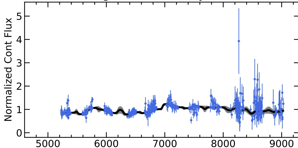
RM553 Light Curves (w/ PyROA model)
