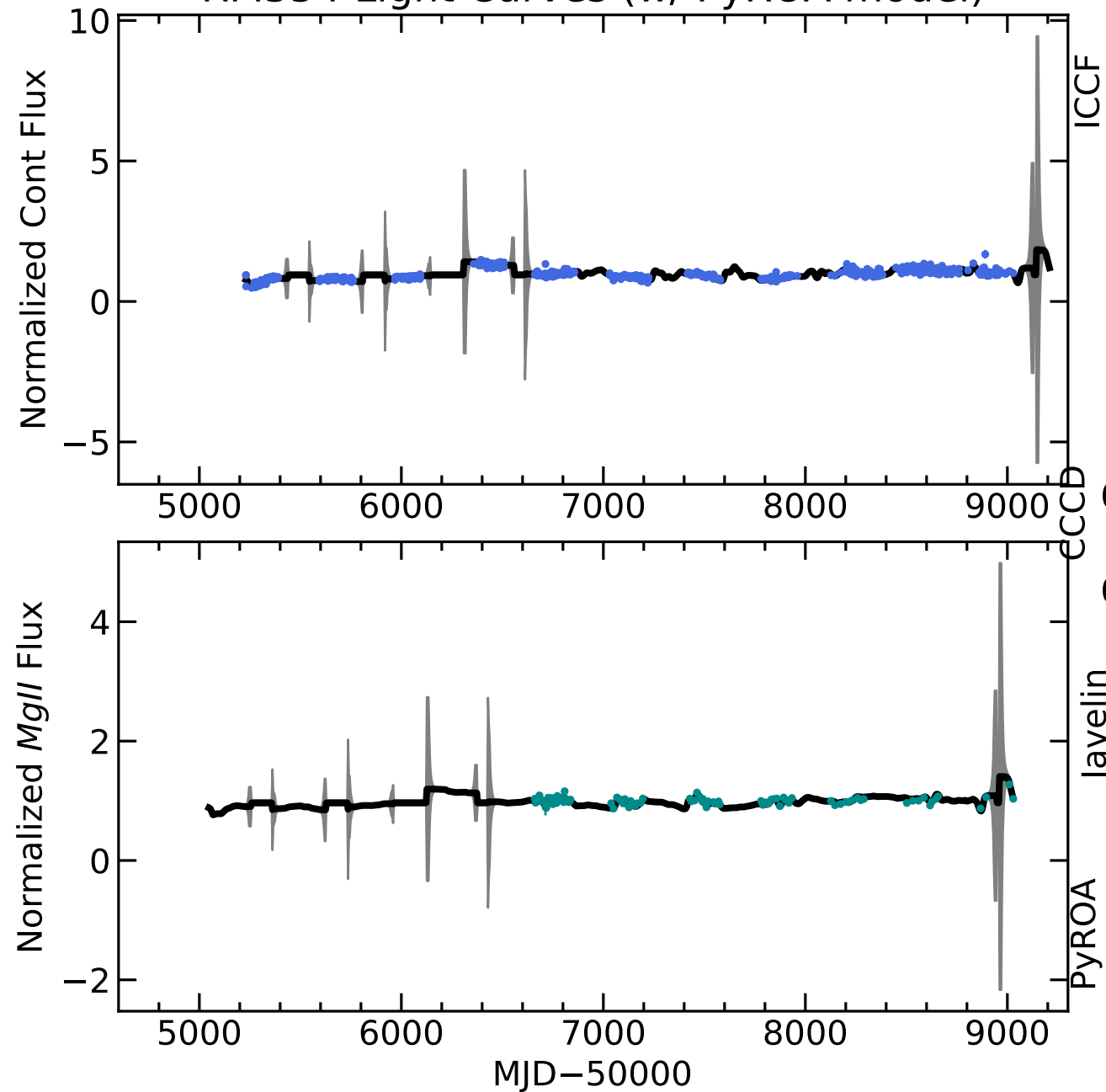
RM554 Light Curves (w/ PyROA model)
