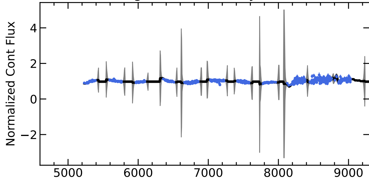
RM555 Light Curves (w/ PyROA model)
