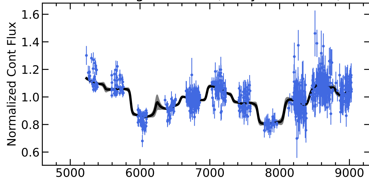
RM556 Light Curves (w/ PyROA model)
