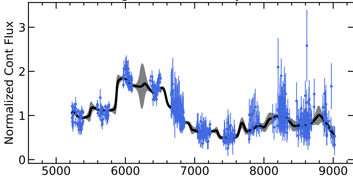
RM559 Light Curves (w/ PyROA model)
