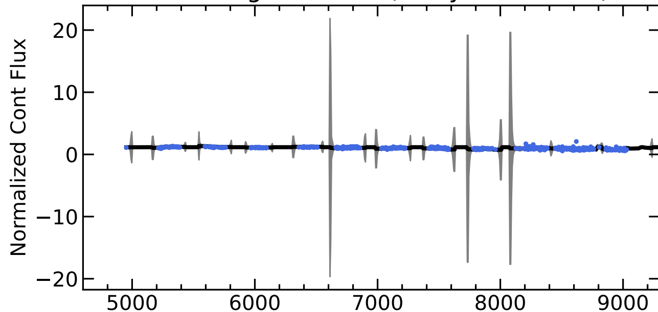
RM562 Light Curves (w/ PyROA model)
