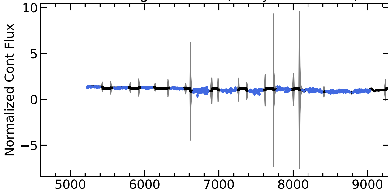
RM564 Light Curves (w/ PyROA model)
