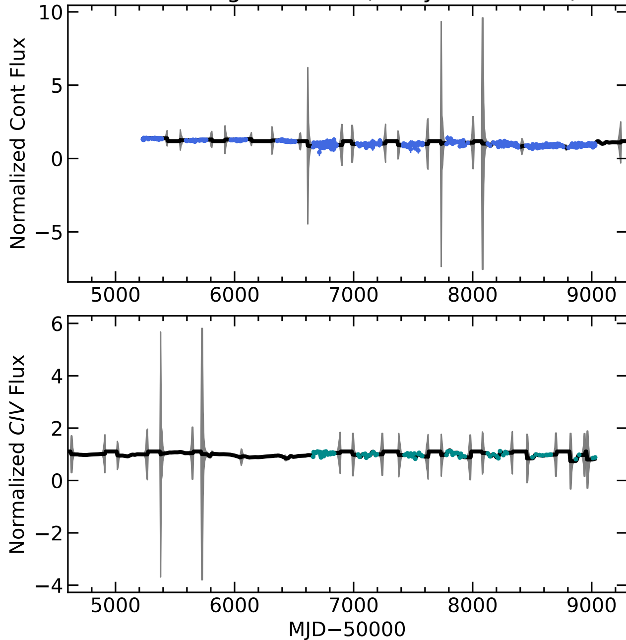
RM564 Light Curves (w/ PyROA model)
