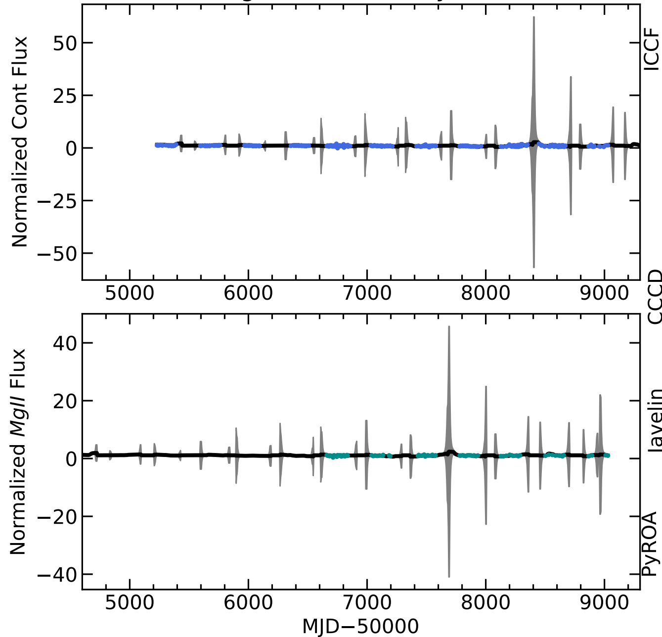
RM566 Light Curves (w/ PyROA model)
