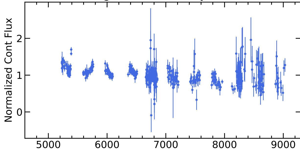
RM566 Light Curves (w/ PyROA model)
