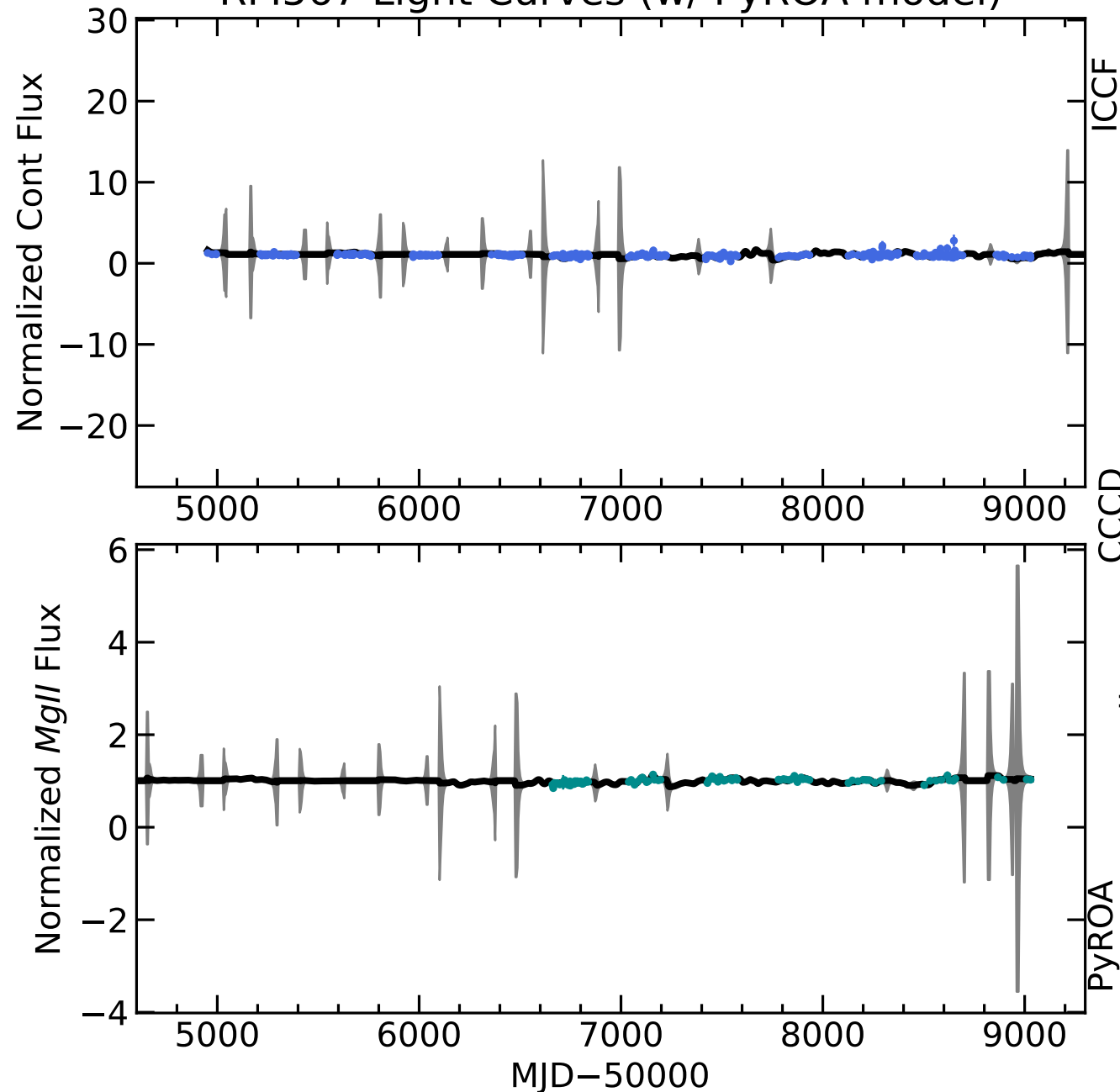
RM567 Light Curves (w/ PyROA model)
