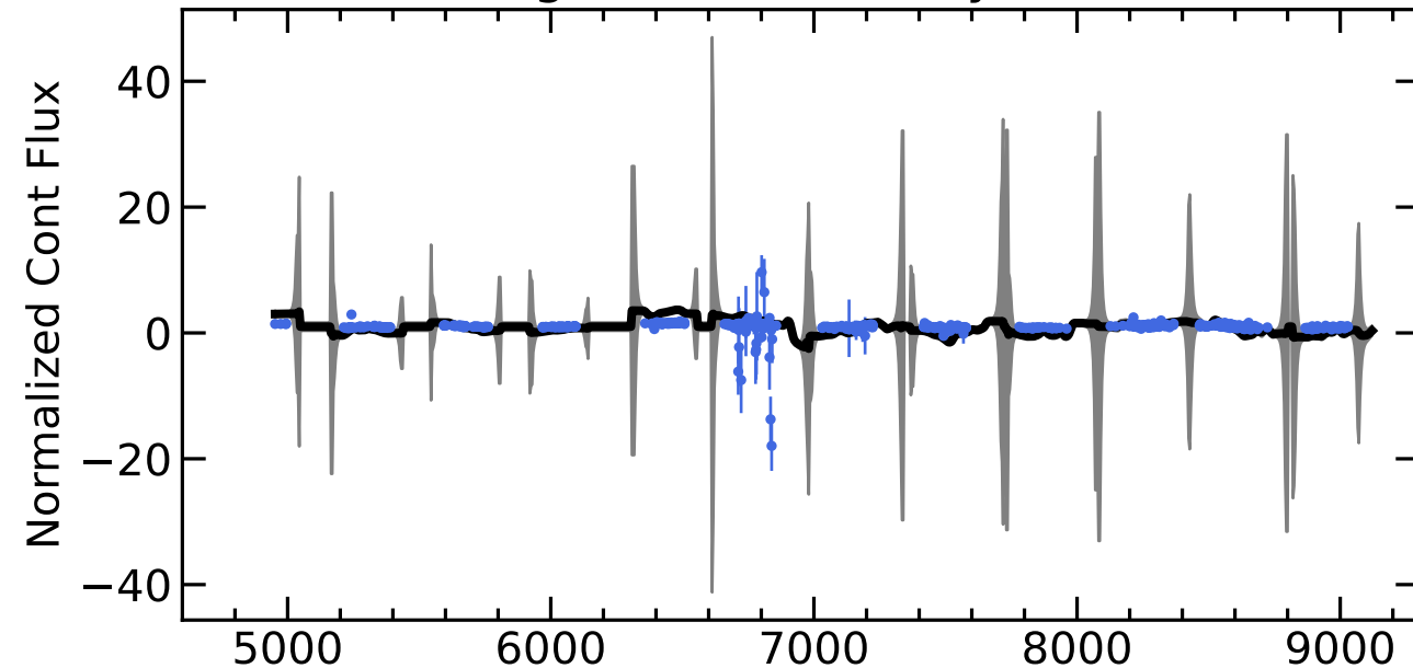
RM568 Light Curves (w/ PyROA model)
