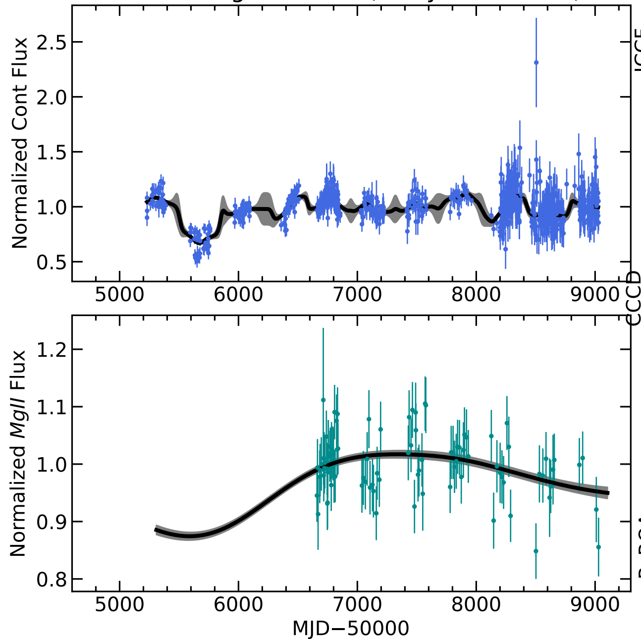
RM569 Light Curves (w/ PyROA model)
