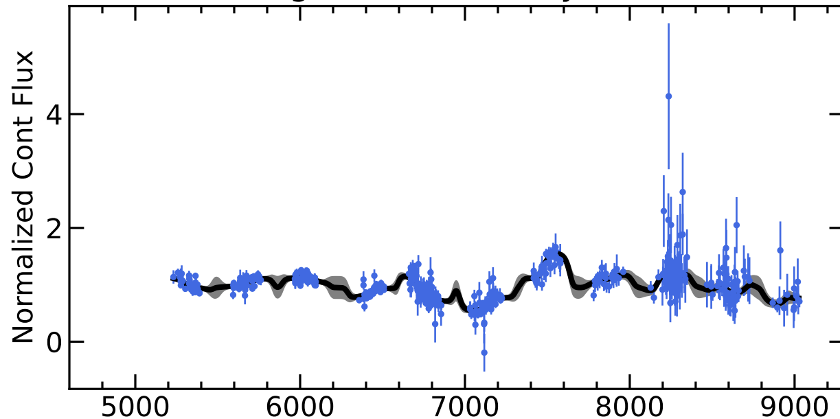
RM570 Light Curves (w/ PyROA model)
