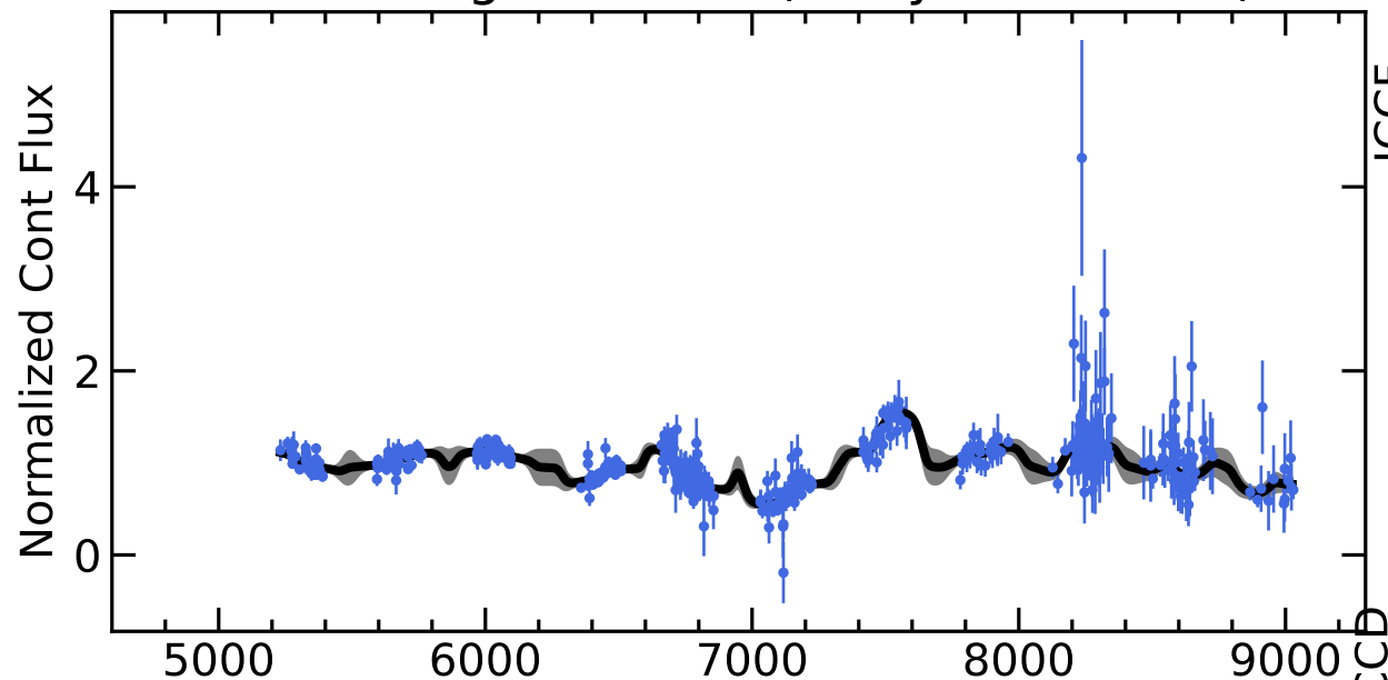
RM570 Light Curves (w/ PyROA model)
