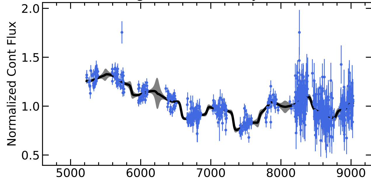
RM572 Light Curves (w/ PyROA model)
