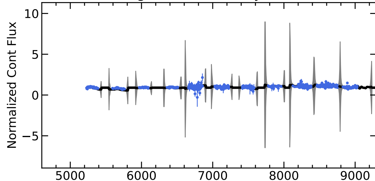
RM573 Light Curves (w/ PyROA model)
