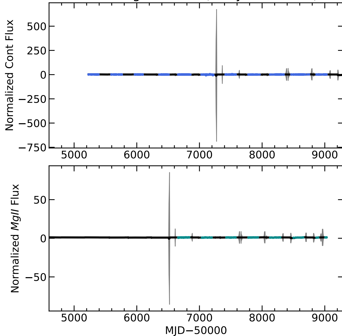
RM574 Light Curves (w/ PyROA model)
