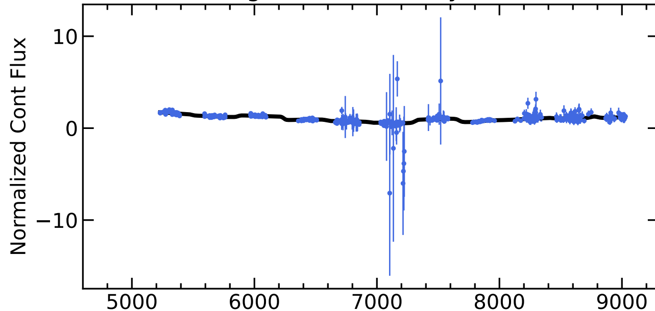
RM574 Light Curves (w/ PyROA model)
