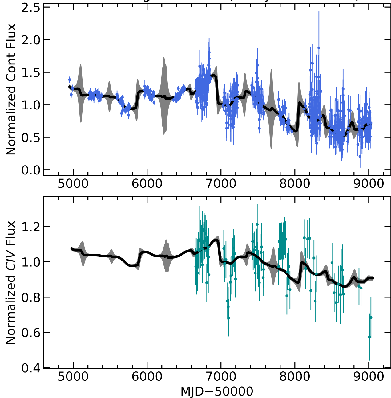
RM575 Light Curves (w/ PyROA model)
