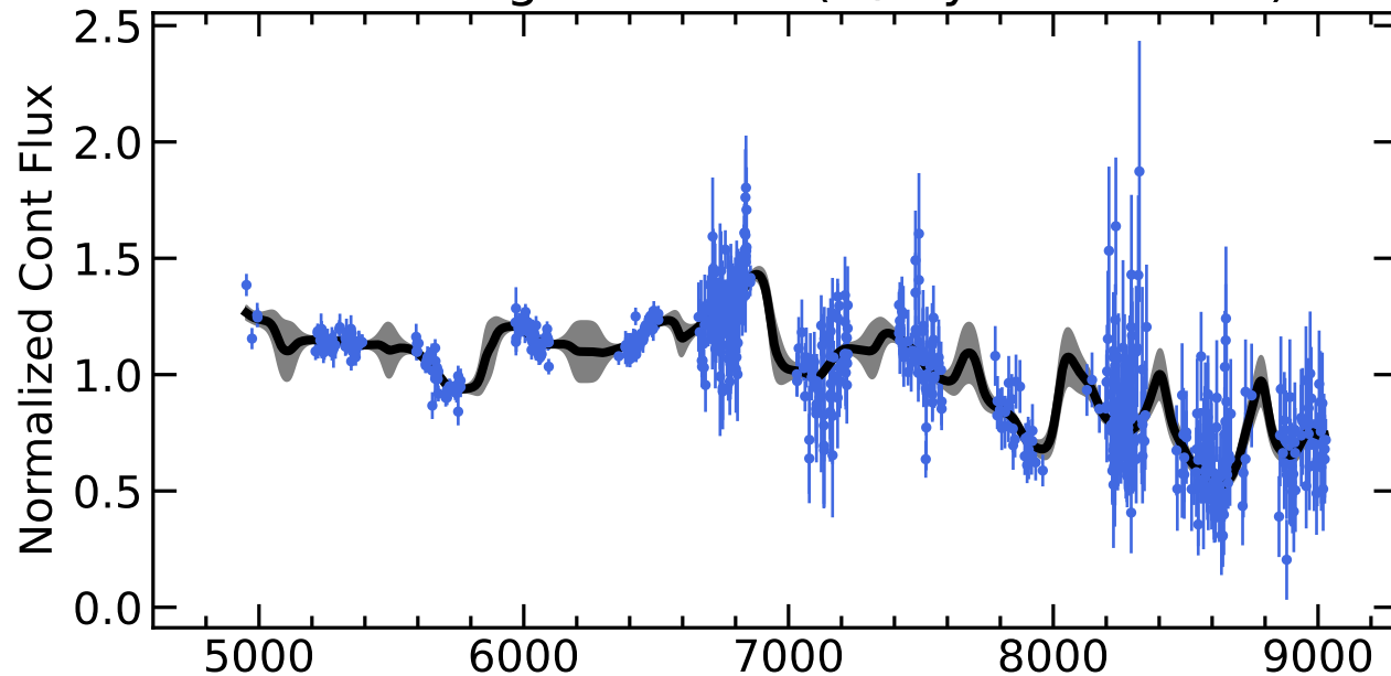
RM575 Light Curves (w/ PyROA model)
