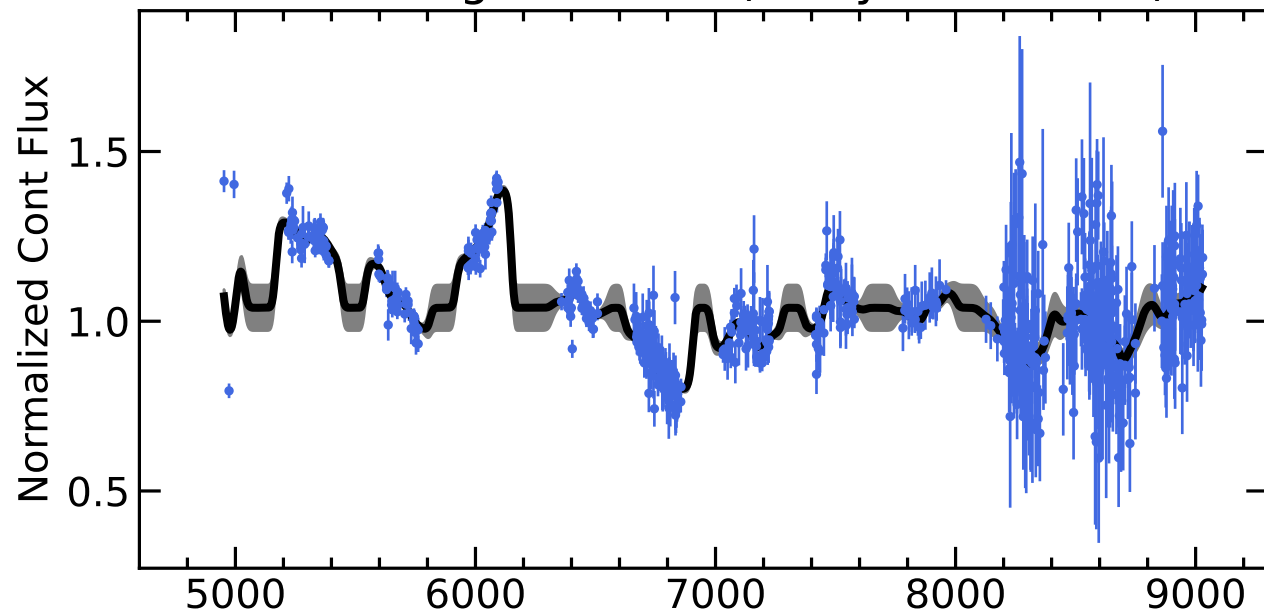
RM576 Light Curves (w/ PyROA model)
