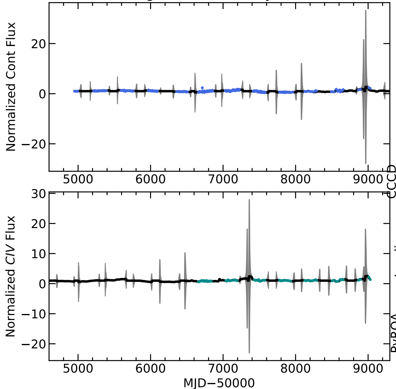
RM579 Light Curves (w/ PyROA model)
