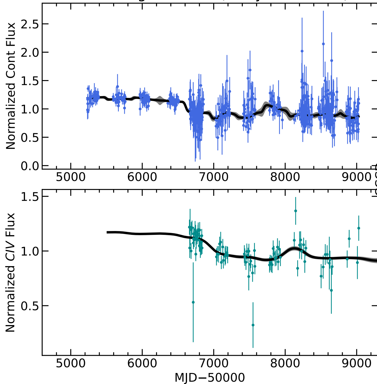
RM580 Light Curves (w/ PyROA model)
