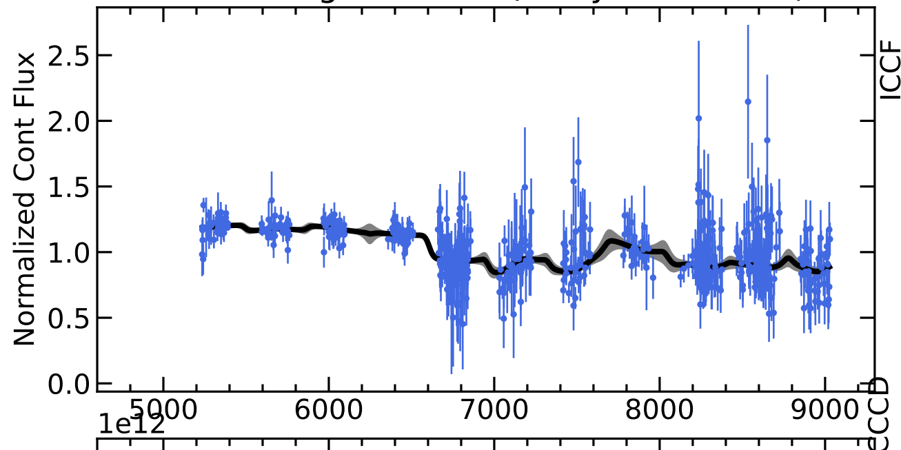
RM580 Light Curves (w/ PyROA model)
