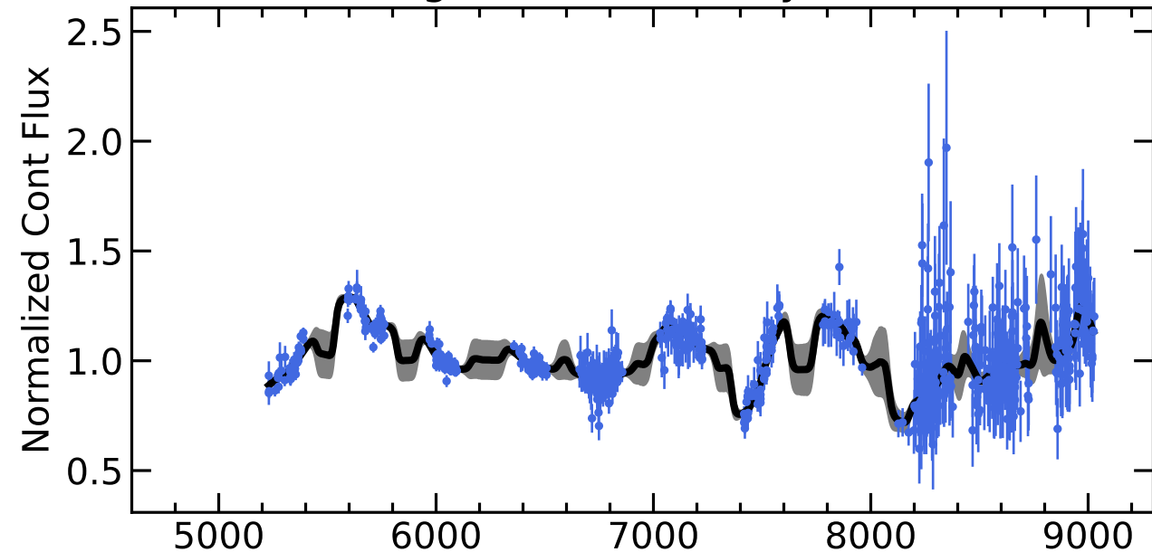
RM581 Light Curves (w/ PyROA model)
