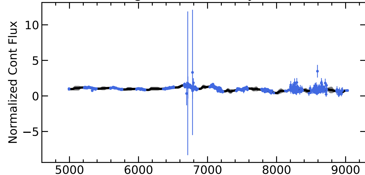
RM583 Light Curves (w/ PyROA model)
