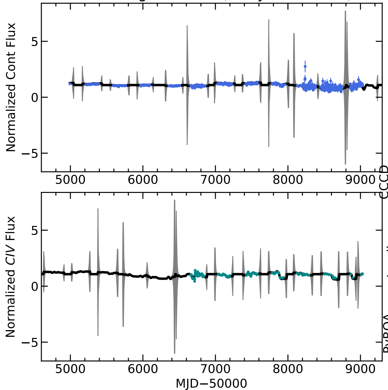
RM584 Light Curves (w/ PyROA model)
