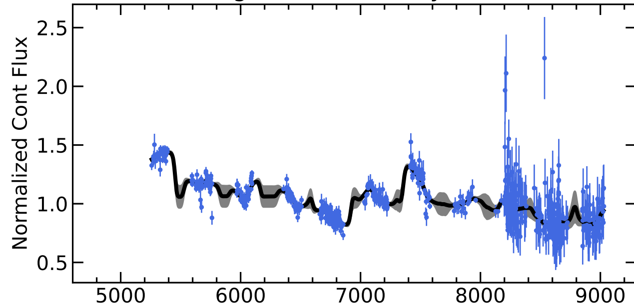
RM585 Light Curves (w/ PyROA model)
