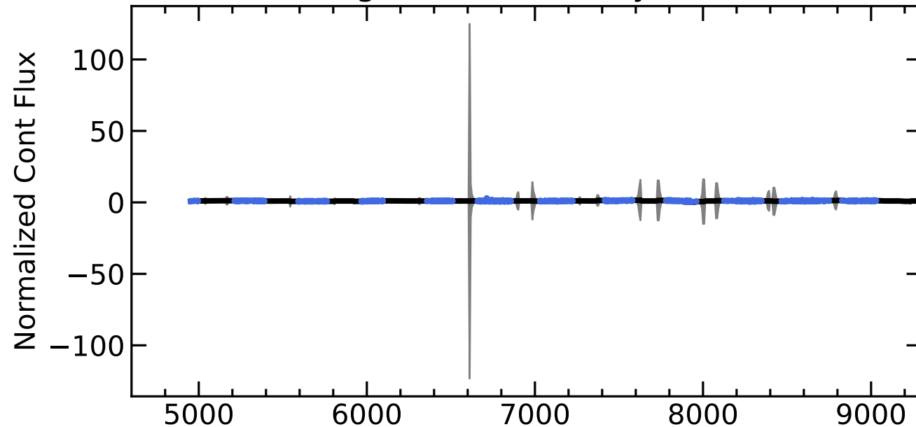
RM586 Light Curves (w/ PyROA model)
