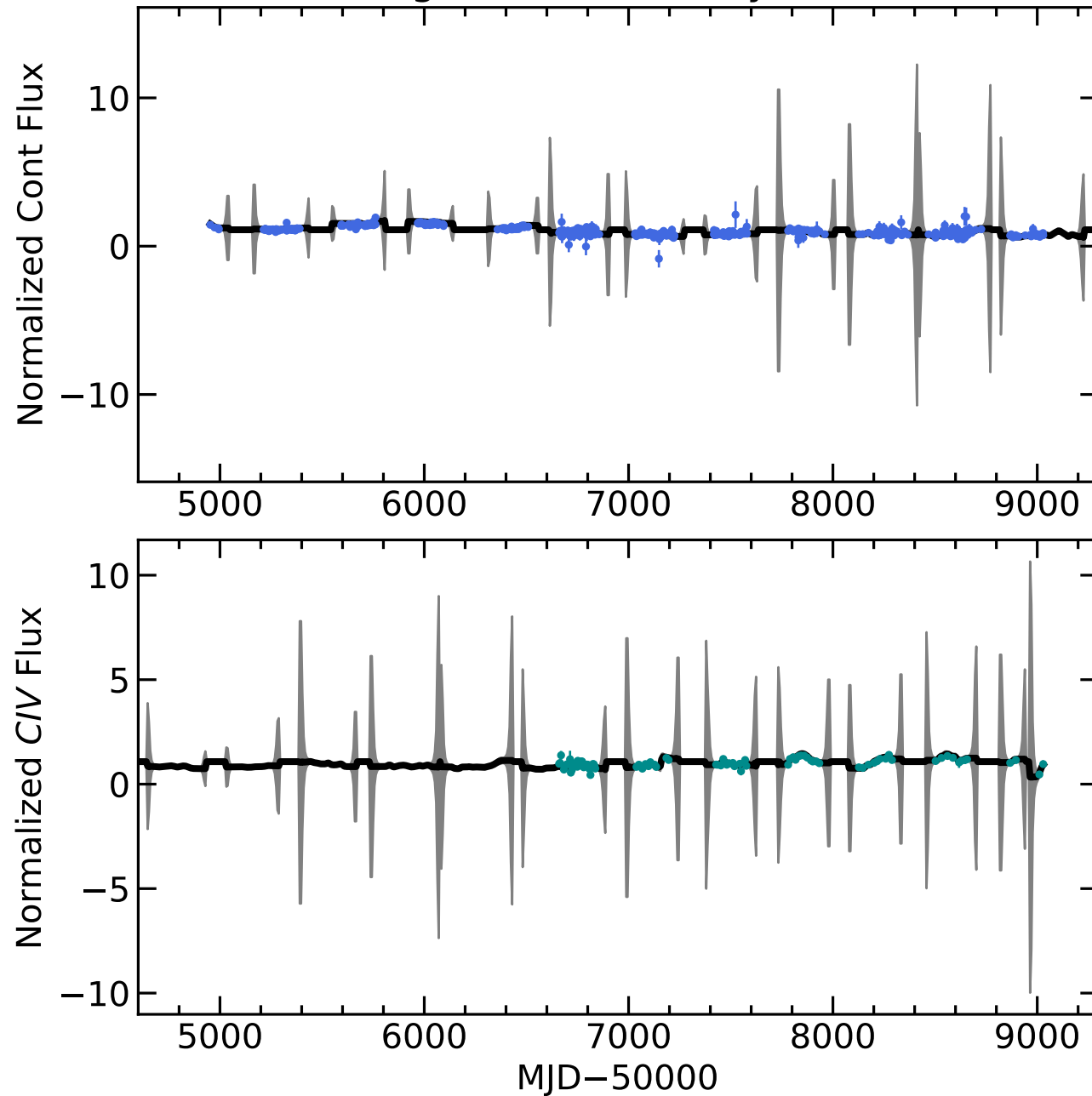
RM587 Light Curves (w/ PyROA model)
