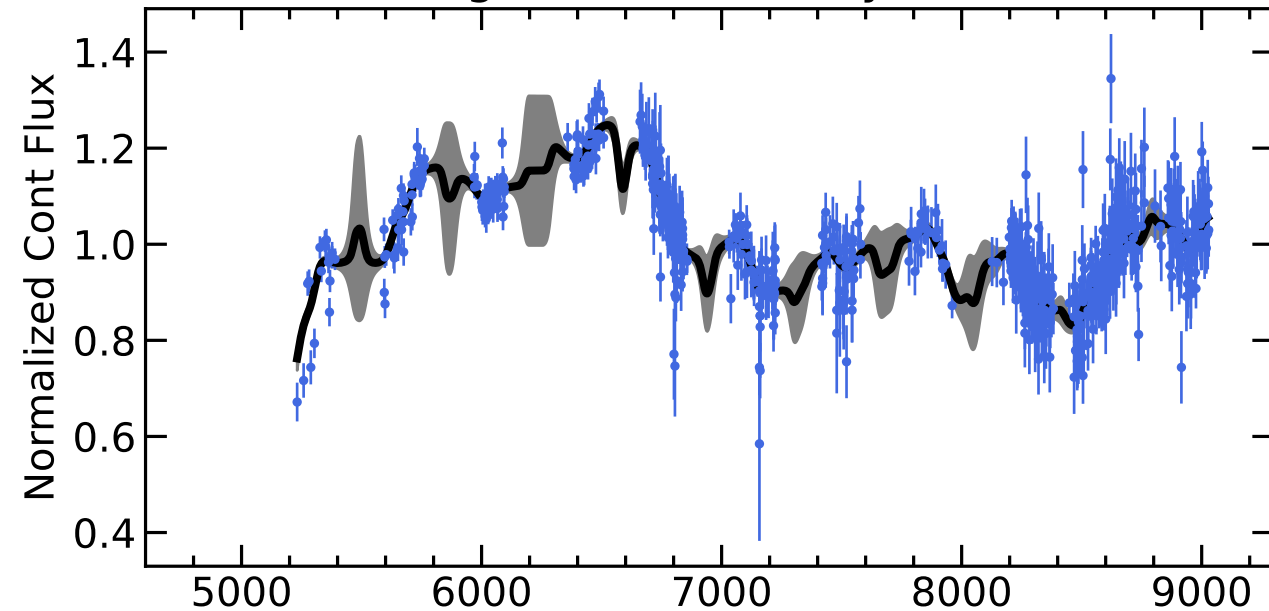
RM588 Light Curves (w/ PyROA model)
