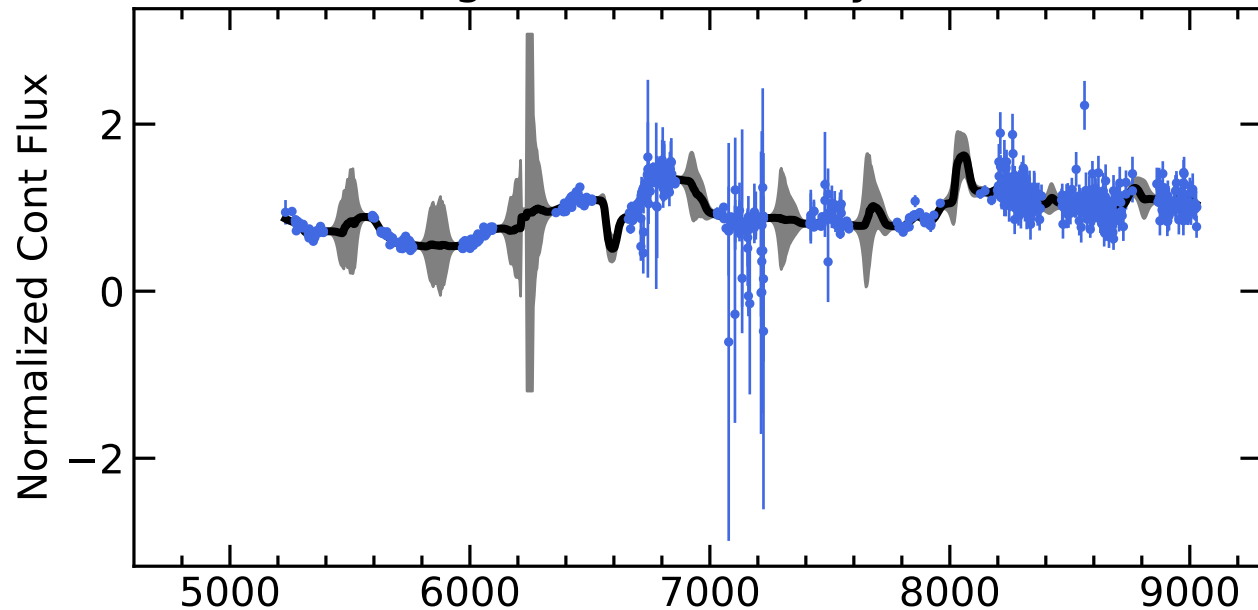
RM589 Light Curves (w/ PyROA model)
