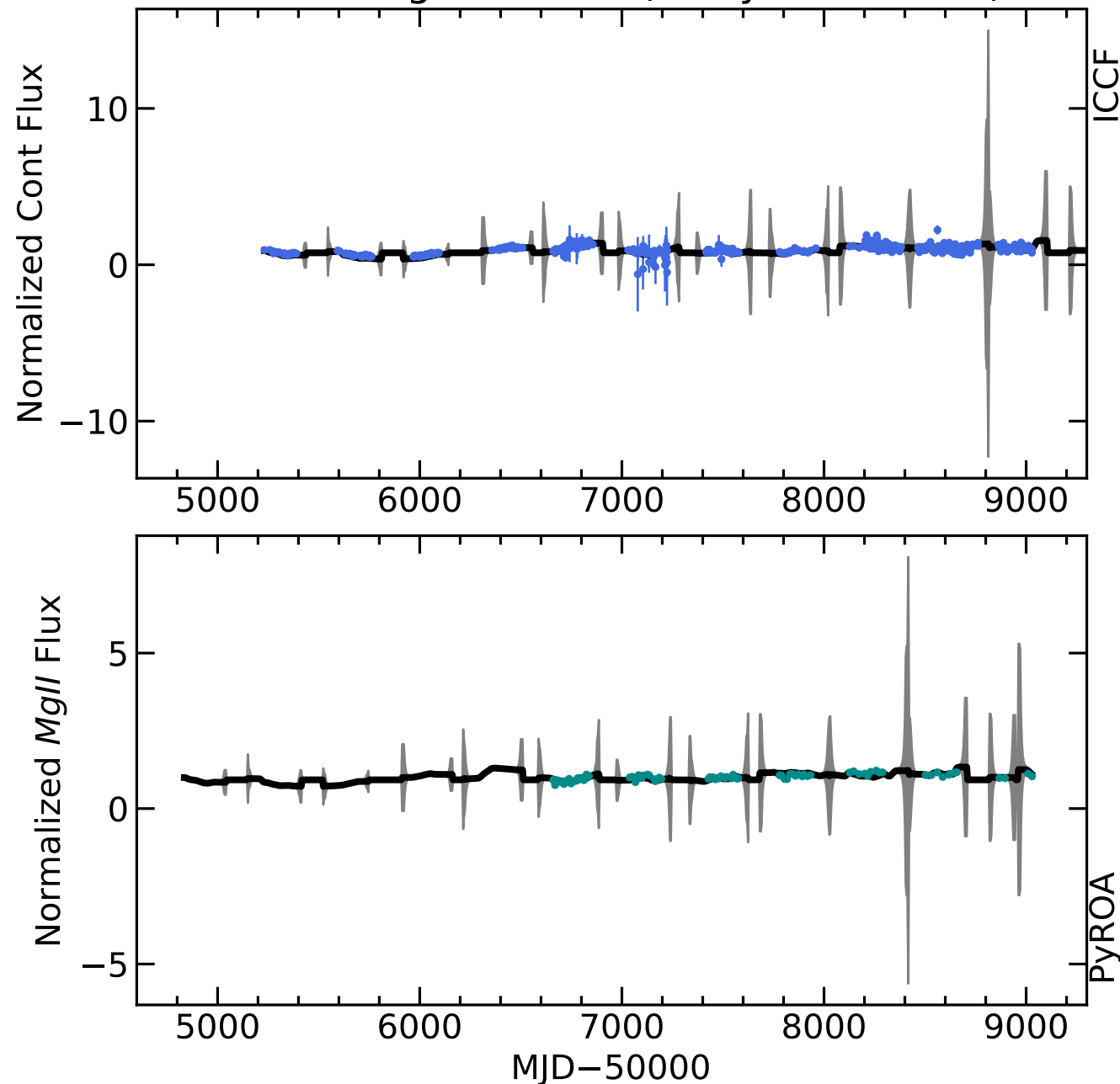
RM589 Light Curves (w/ PyROA model)
