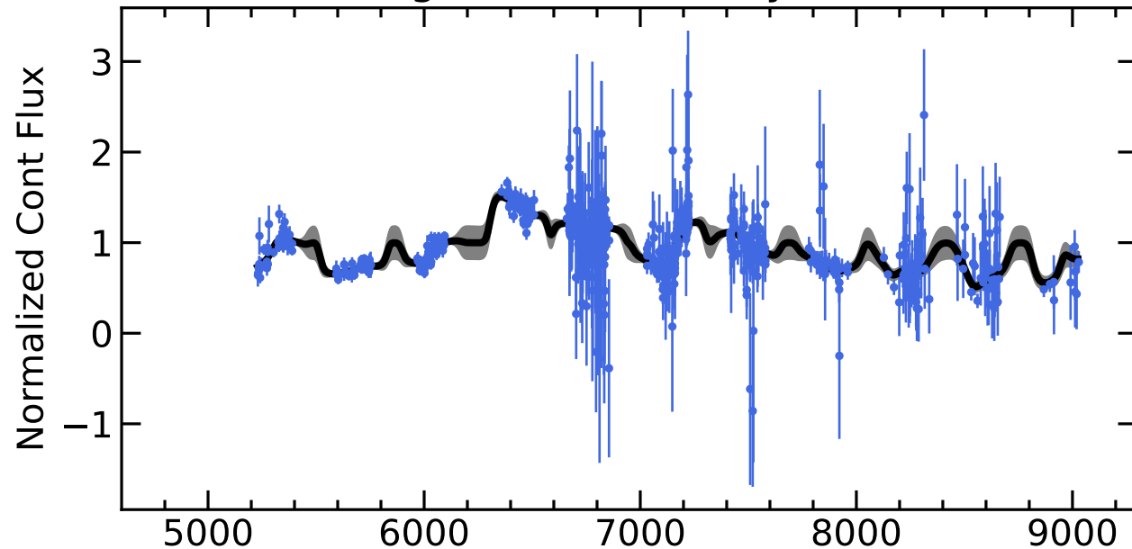
RM590 Light Curves (w/ PyROA model)
