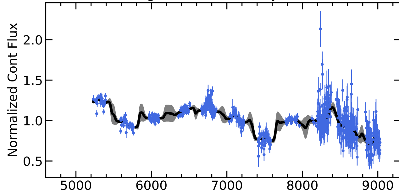
RM593 Light Curves (w/ PyROA model)
