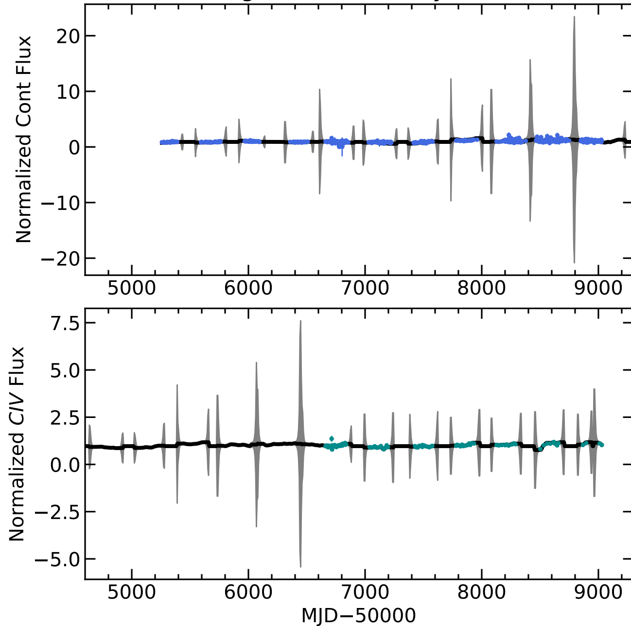
RM594 Light Curves (w/ PyROA model)
