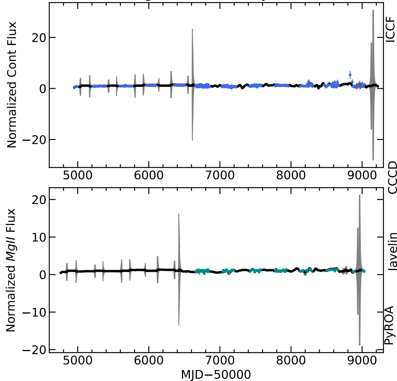
RM595 Light Curves (w/ PyROA model)
