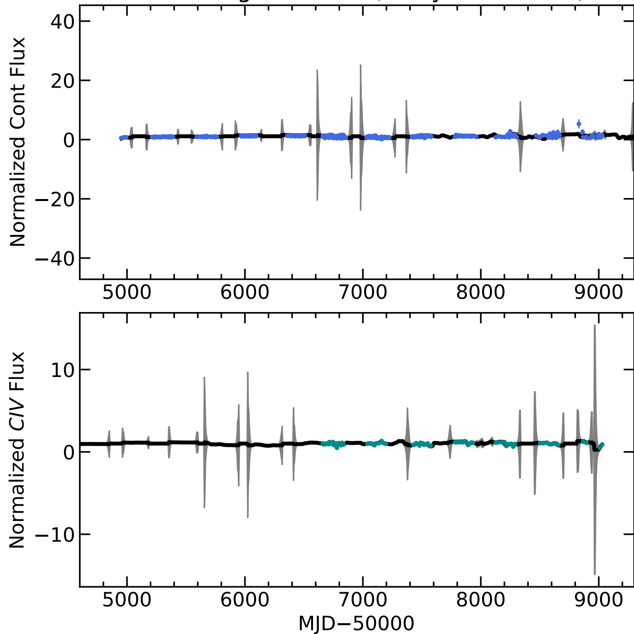
RM595 Light Curves (w/ PyROA model)
