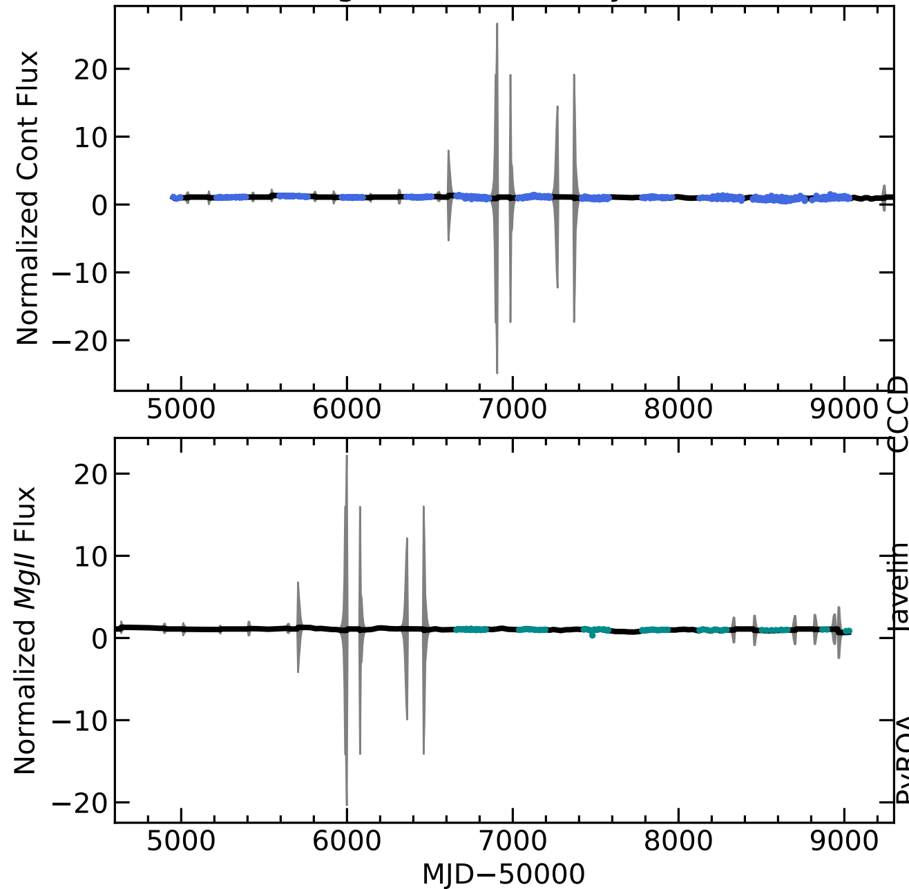
RM596 Light Curves (w/ PyROA model)
