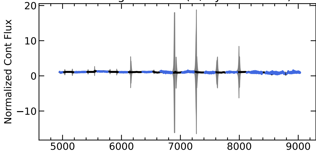
RM596 Light Curves (w/ PyROA model)
