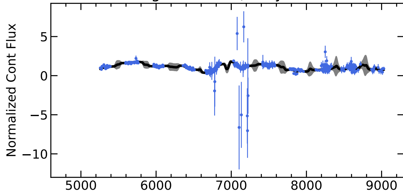
RM597 Light Curves (w/ PyROA model)
