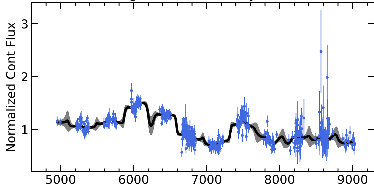
RM599 Light Curves (w/ PyROA model)
