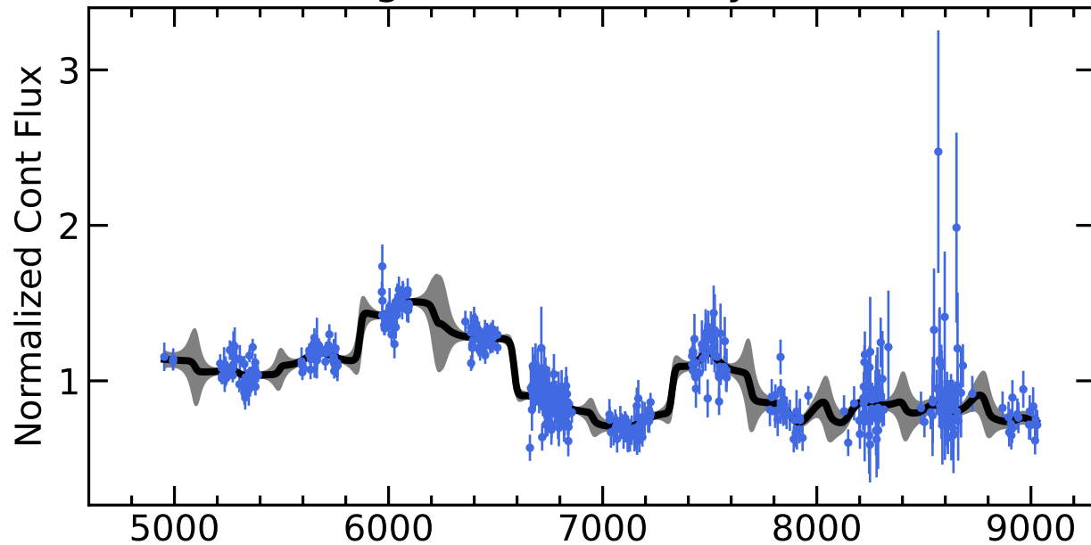
RM599 Light Curves (w/ PyROA model)
