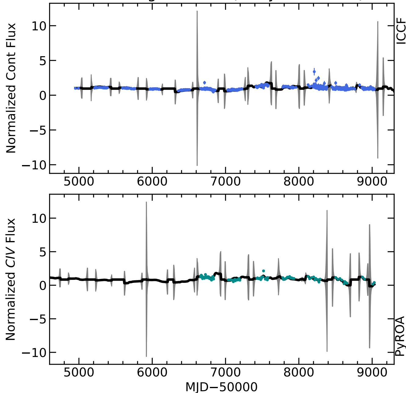
RM600 Light Curves (w/ PyROA model)
