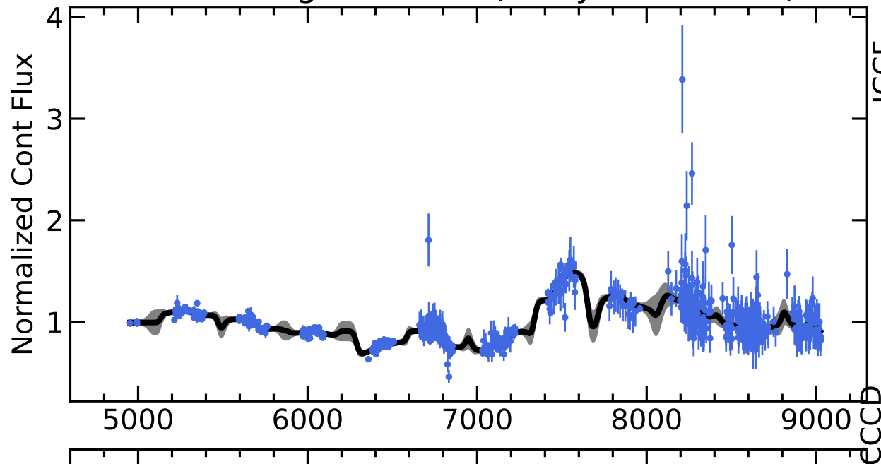
RM600 Light Curves (w/ PyROA model)
